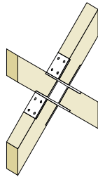
Thorncross Chapel Custom Joint - Roof Truss Joint - Screwed
