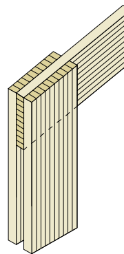
Knee Joint - Glued Cross Lap
