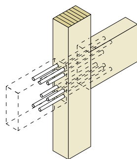
Beam-Column Joint - Epoxied Bars
