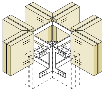
Deep Beam-Grid - Welded Joint Plate
