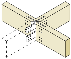
Beam-Grid - Welded Joint Plate
