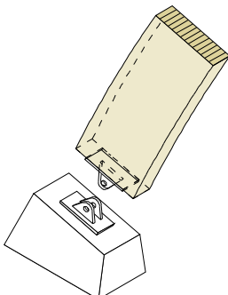
Foot Joint - Exposed Pin Joint
