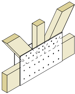
Truss Joint - Side Gusset Plates
