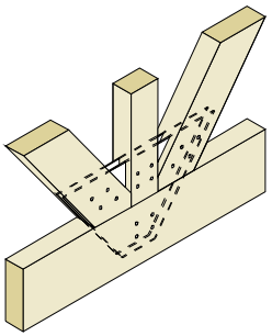
Truss Joint - Internal Metal Gusset Plate
