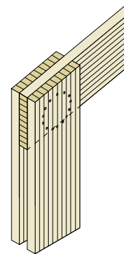
Knee Joint - Mechanically Fastened Cross Lap with Pressed-in Metal Dowels
