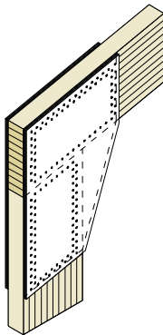
Knee Joint - Nailed Plywood Gussets
