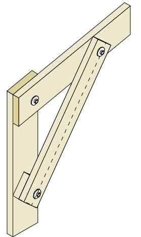
Knee Joint - Bolt Fixed Triangulated Brace
