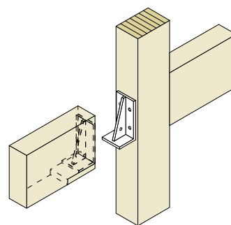
Beam-Column Joint - Steel Hanger with Central Web
