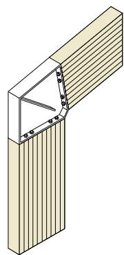
Knee Joint - Epoxied Rods & Steel Connector
